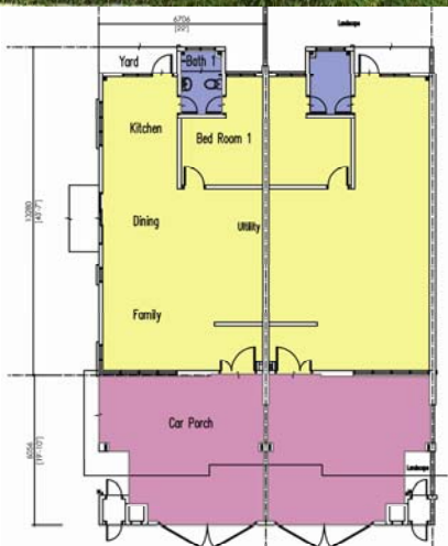
TYPICAL GROUND FLOOR PLAN
