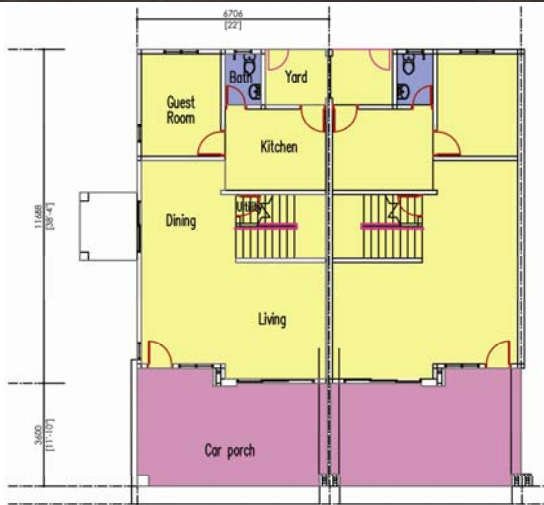
TYPICAL GROUND FLOOR PLAN
