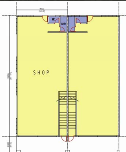
TYPICAL GROUND FLOOR PLAN
